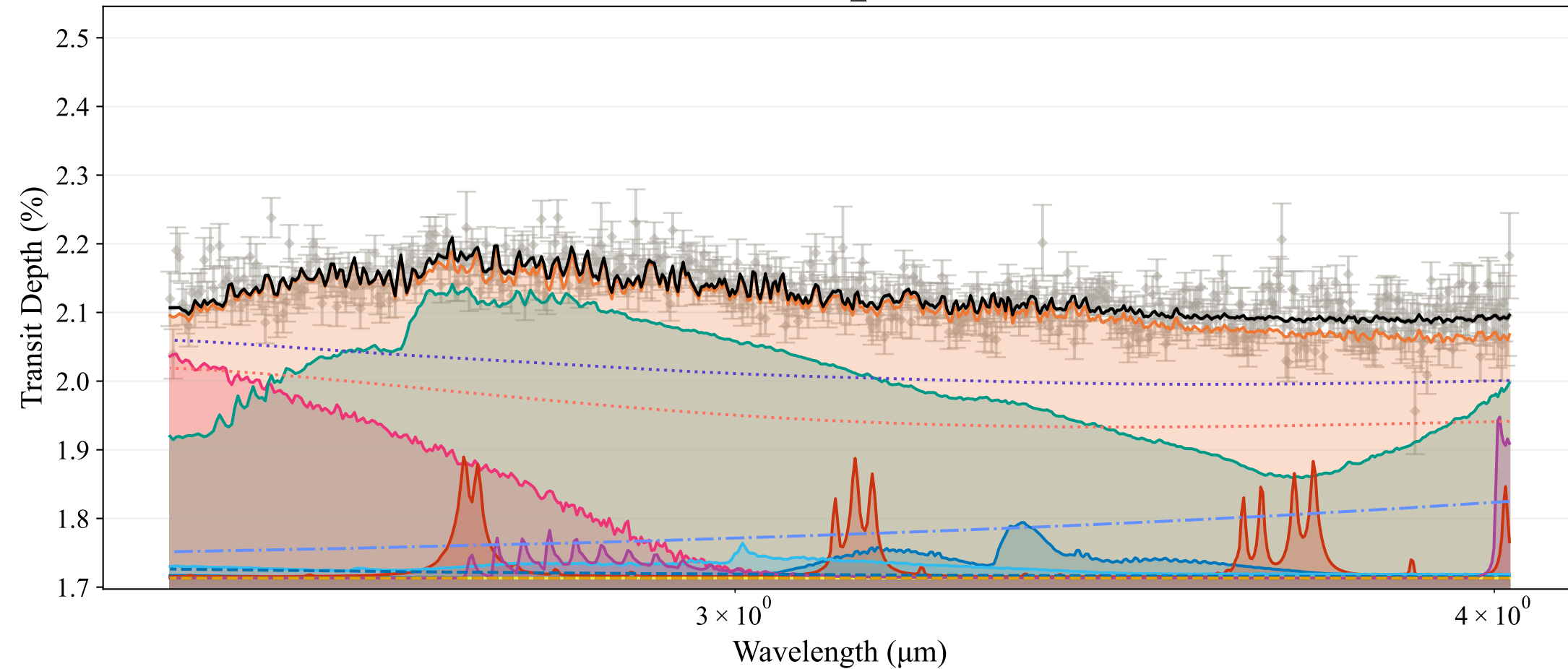
nircam_SiO
